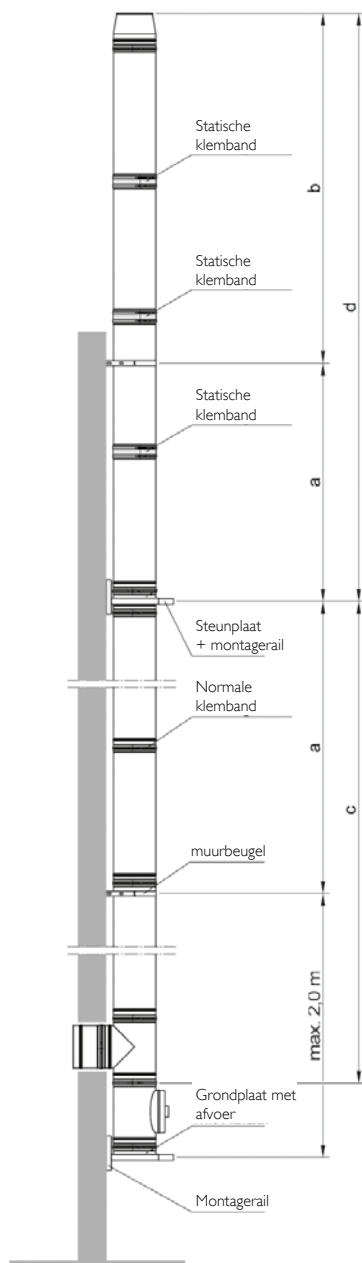
ICS Ø80-400
